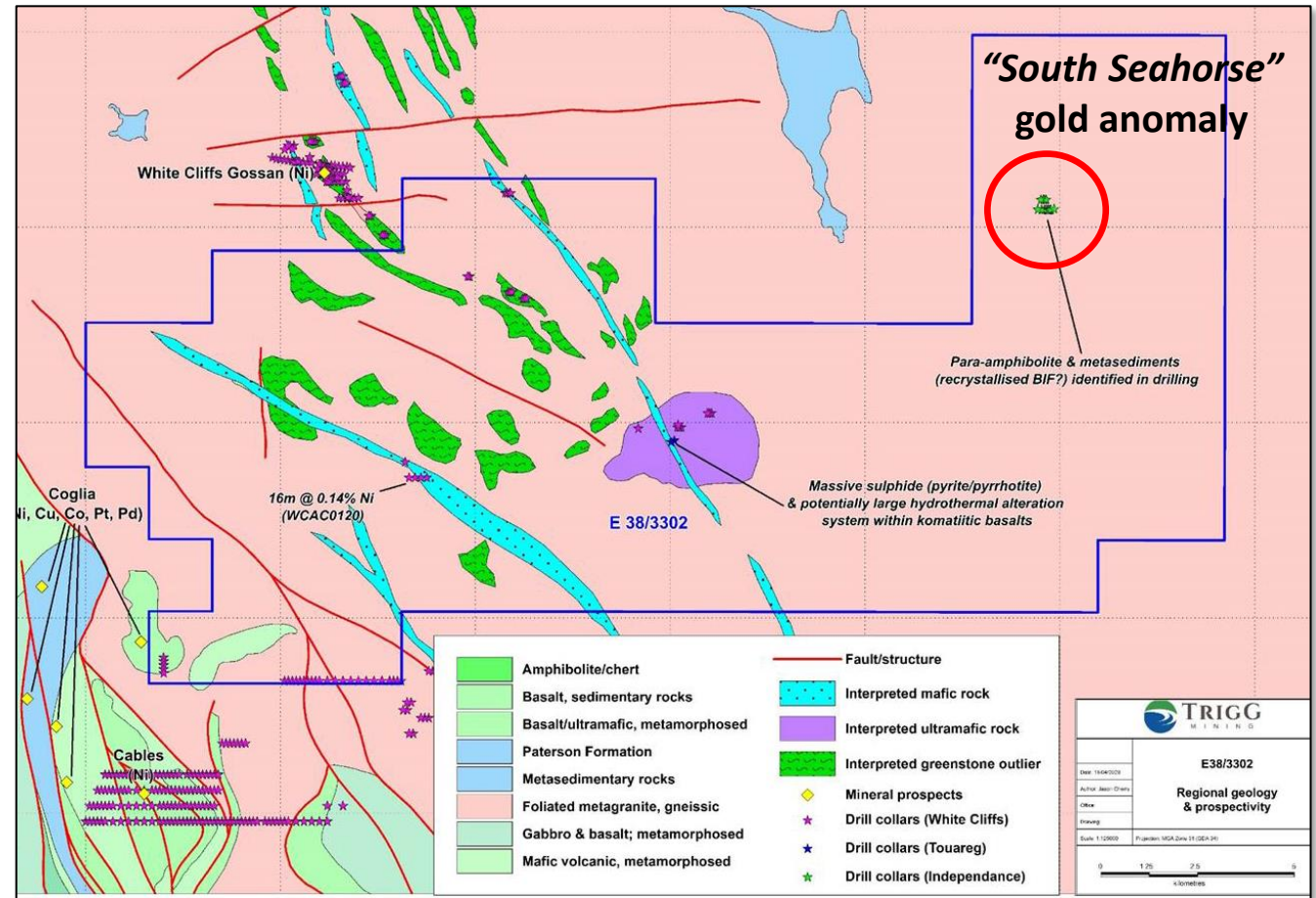
East Laverton Project E38/3302 interpreted geology (Trigg Mining Ltd)
