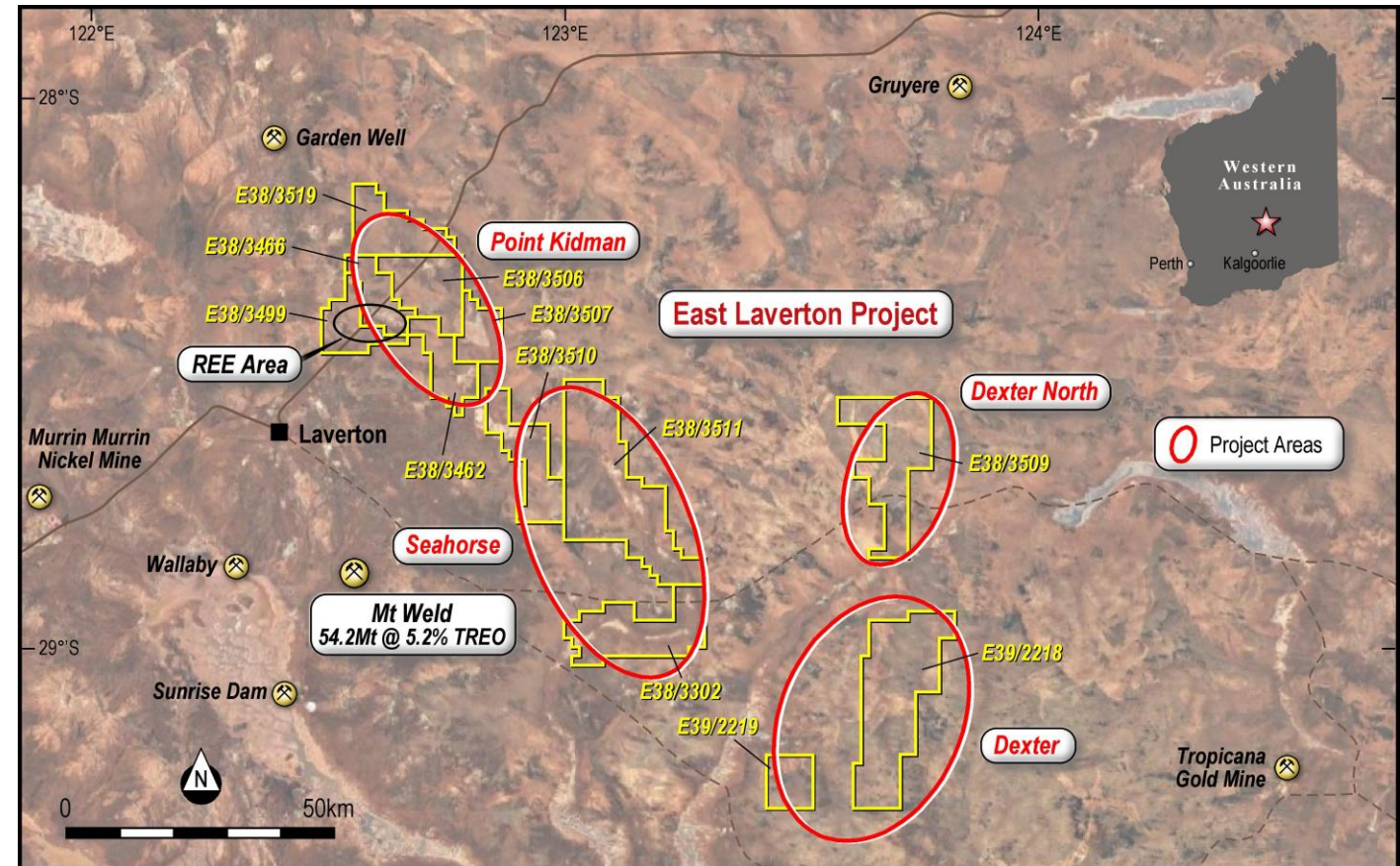
East Laverton Project tenement locations and key prospect areas on surface image
