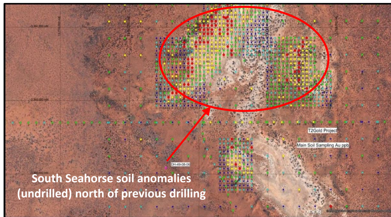
South Seahorse Prospect soil sampling results overlay on surface image
