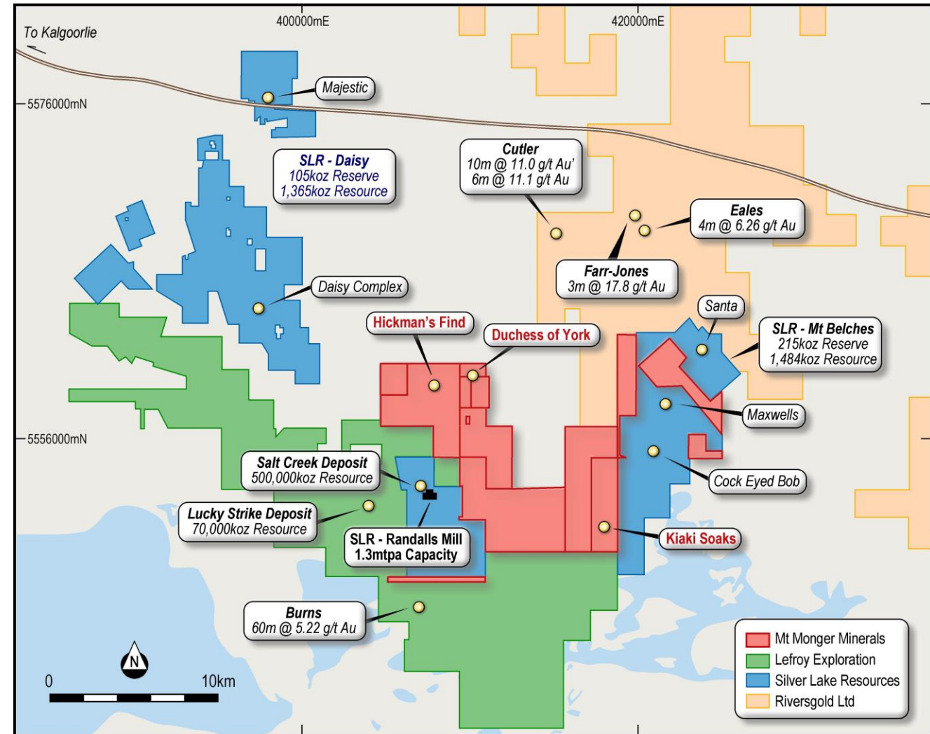
Mt Monger Project selected tenement holdings, gold mines and gold occurrences
