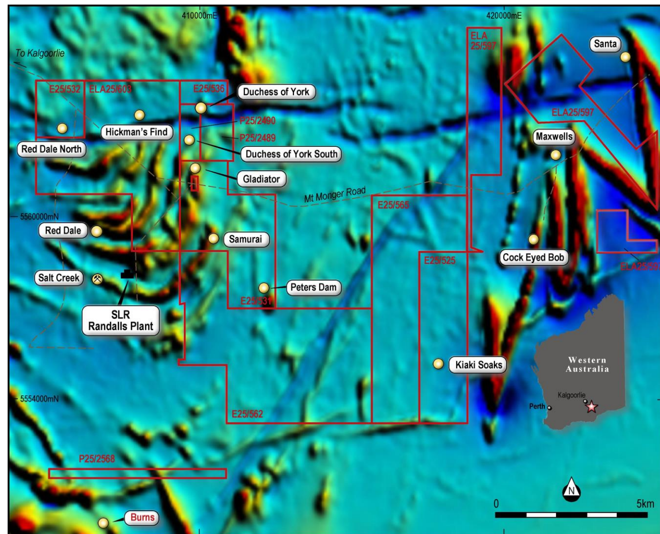
Mt Monger Project regional magnetic image (TMI RTP) showing tenements and prospect areas
